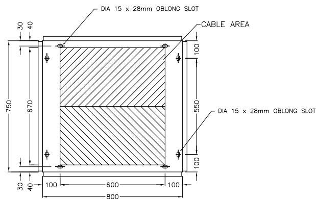
CHANNEL BASE
