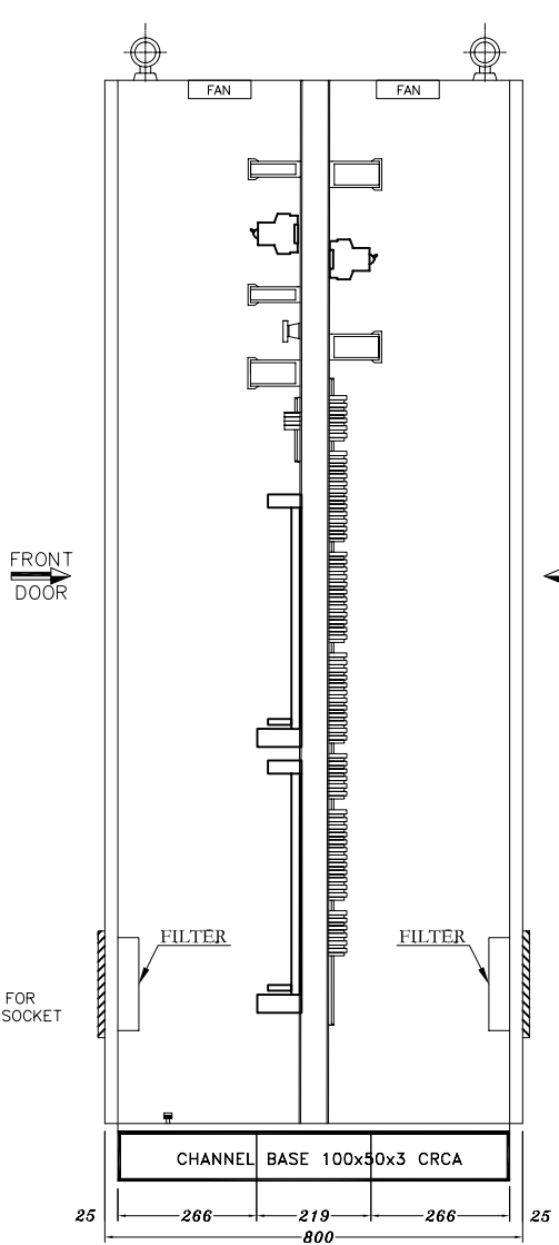
SECTIONAL SIDE VIEW
