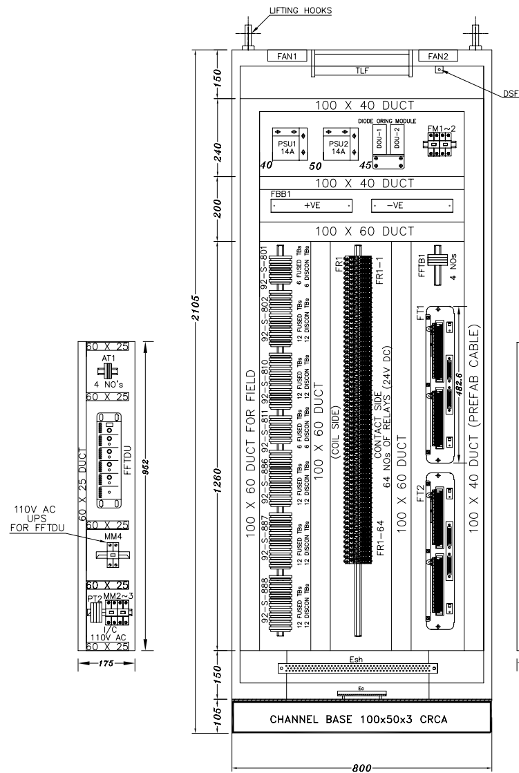
SECTIONAL FRONT VIEW
