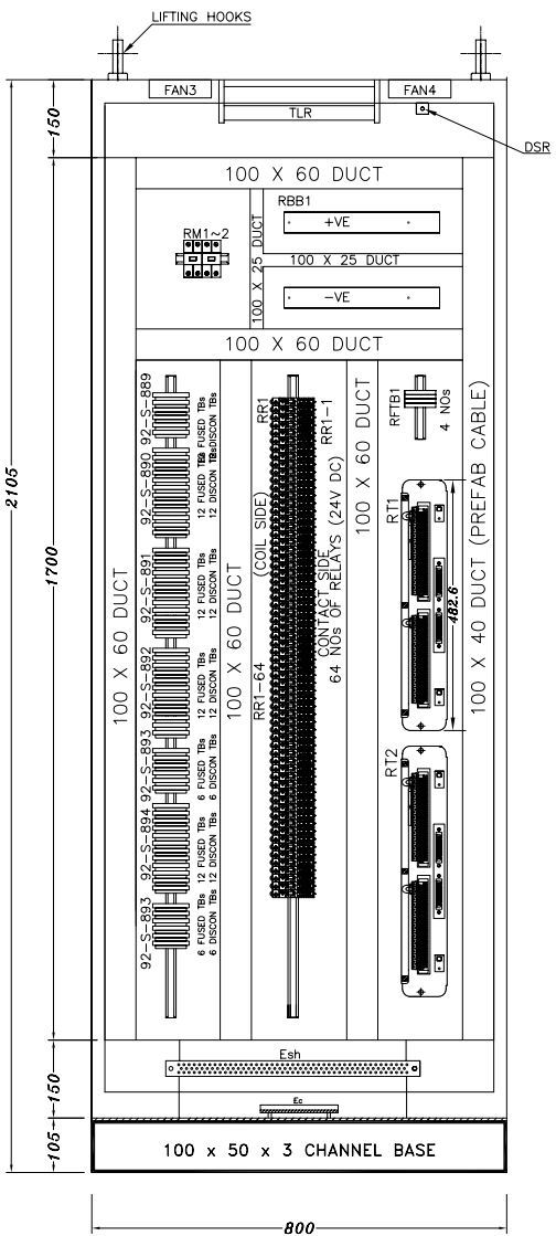
SECTIONAL REAR VIEW
