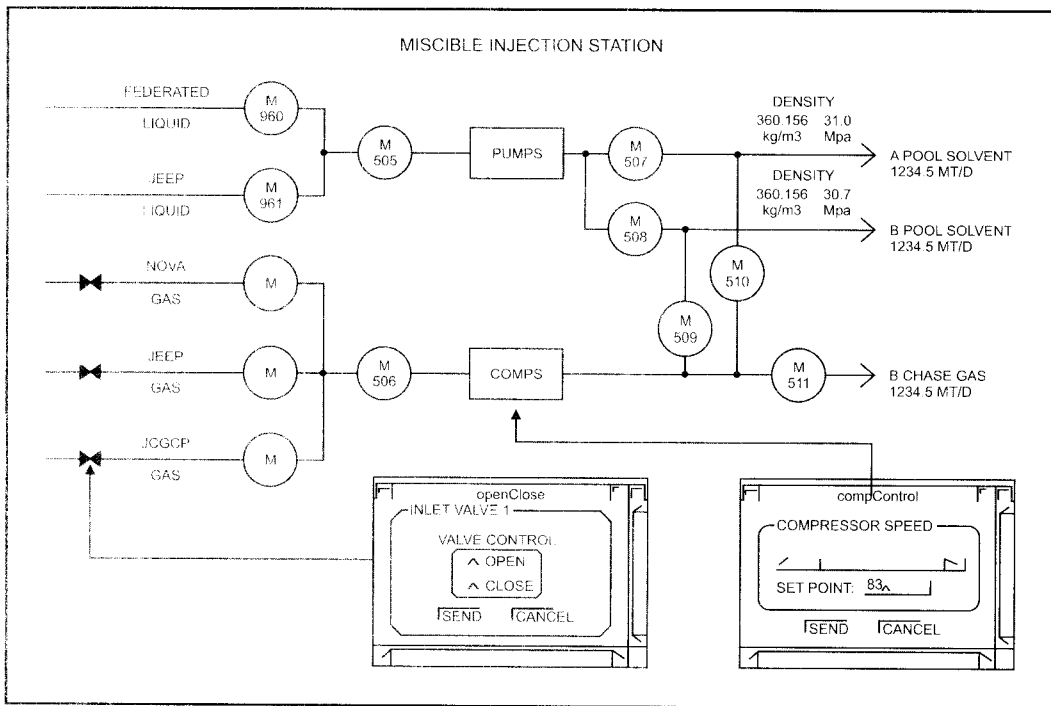
Figure 12-5. Control Screen (Courtesy: TesserNet Systems Inc.)
