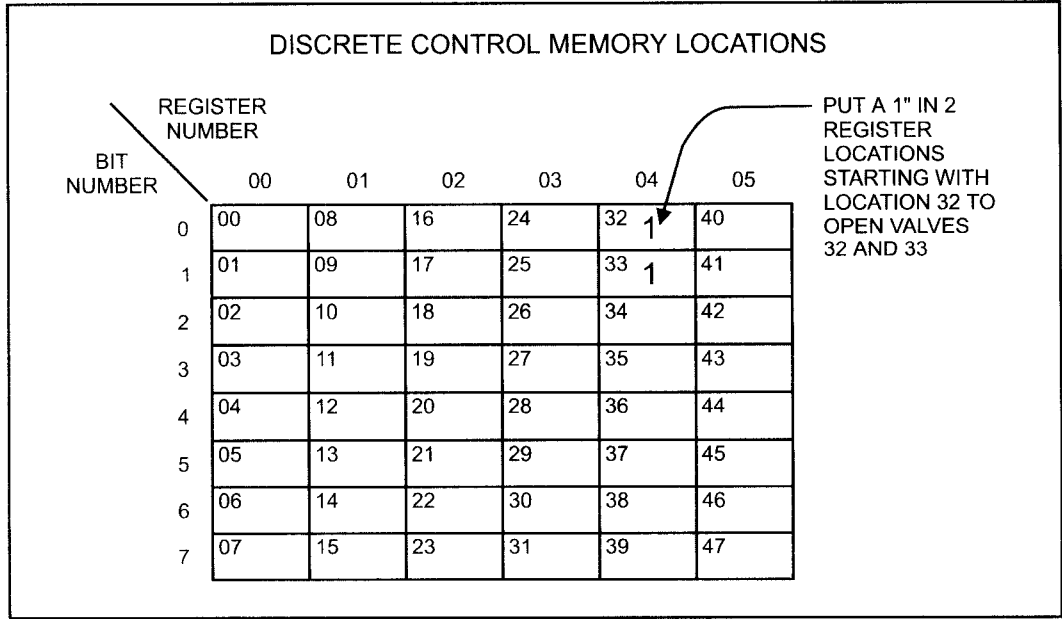
Figure 8-8. Message to RTU Calling for It to Open a Two-position Valve
