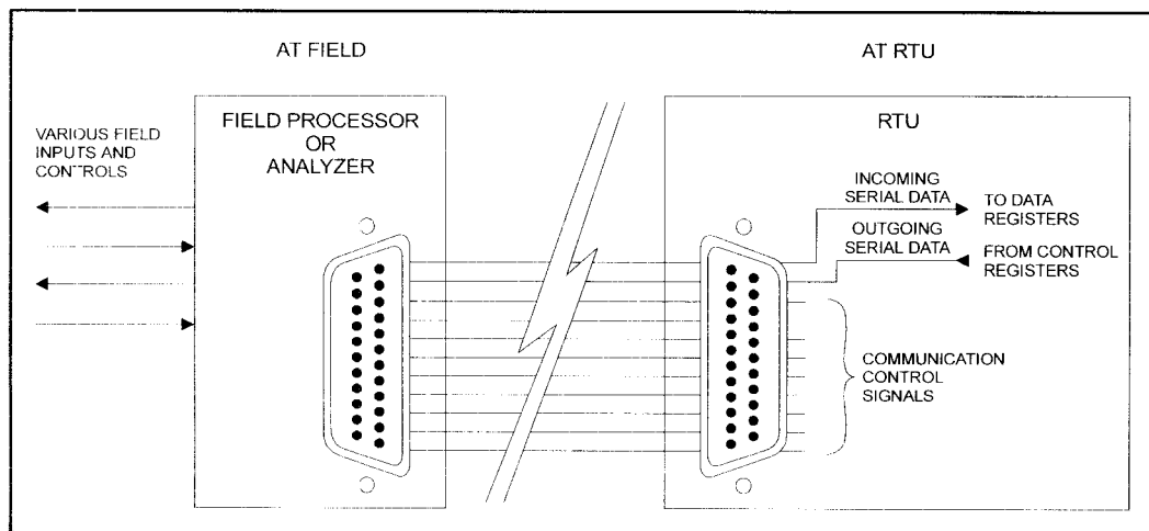
Figure 8-15. RS-232 Link
